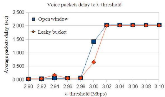
Fig. 4: Average voice packet delay versus threshold rate
