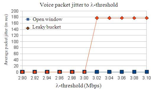
Fig. 5: Average packets jitter versus threshold rate
