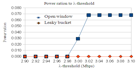
Fig. 11: Power ratio to threshold rate
