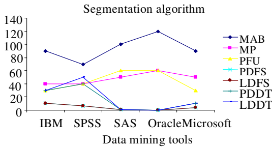
Fig. 4: Performance metrics of data mining tools based on segmentation algorithms
