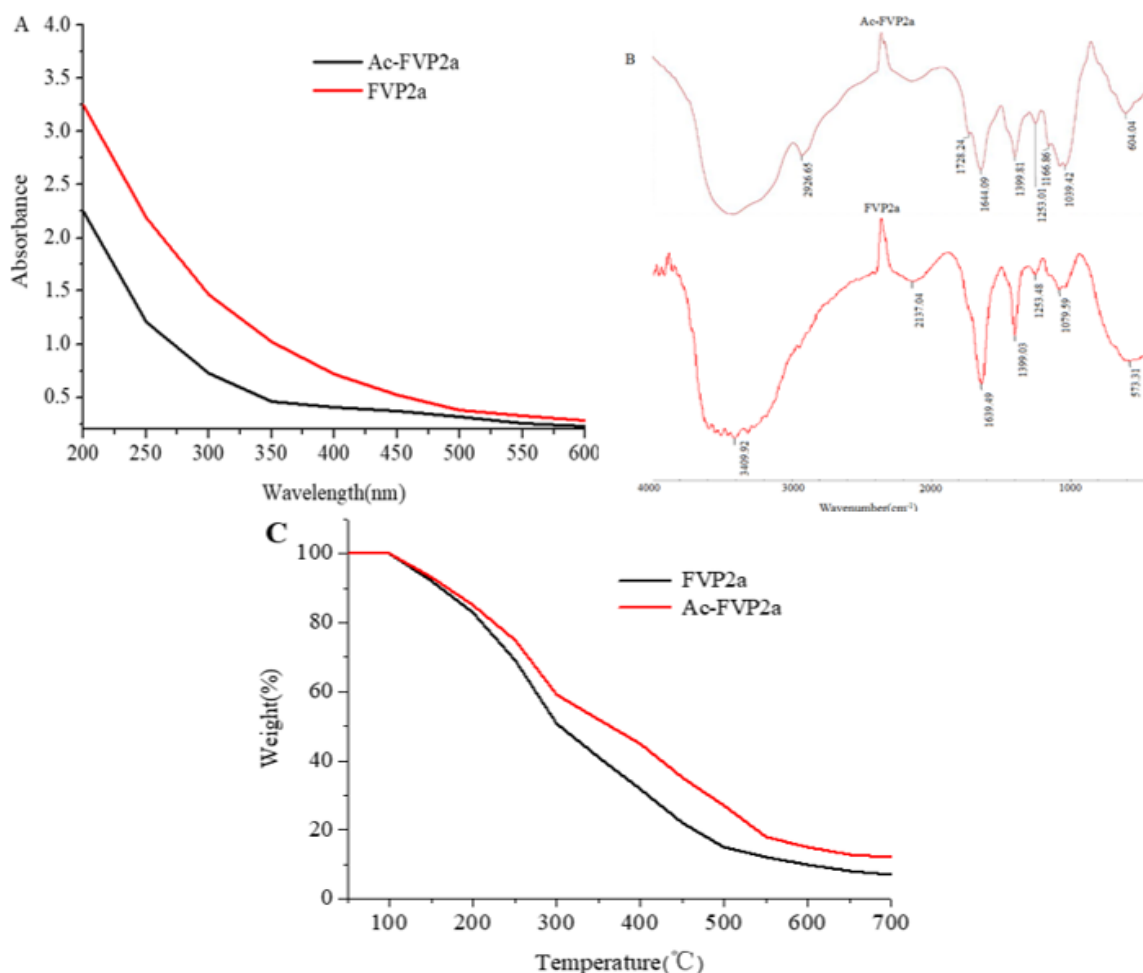
Fig. 2: Characterization of FVP2a and Ac-FVP2a (A: UV-Vis. B: FT-IR. C: Thermogravimetric)
