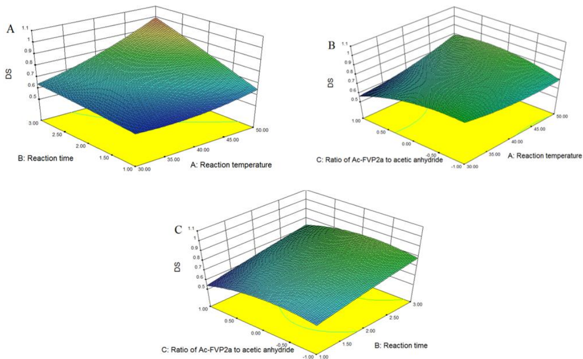
Fig. 1: Effect of cross-interaction of reaction temperature, reaction time, and the ratio of FVP2a to acetic anhydride on DS of Ac-FVP2a
