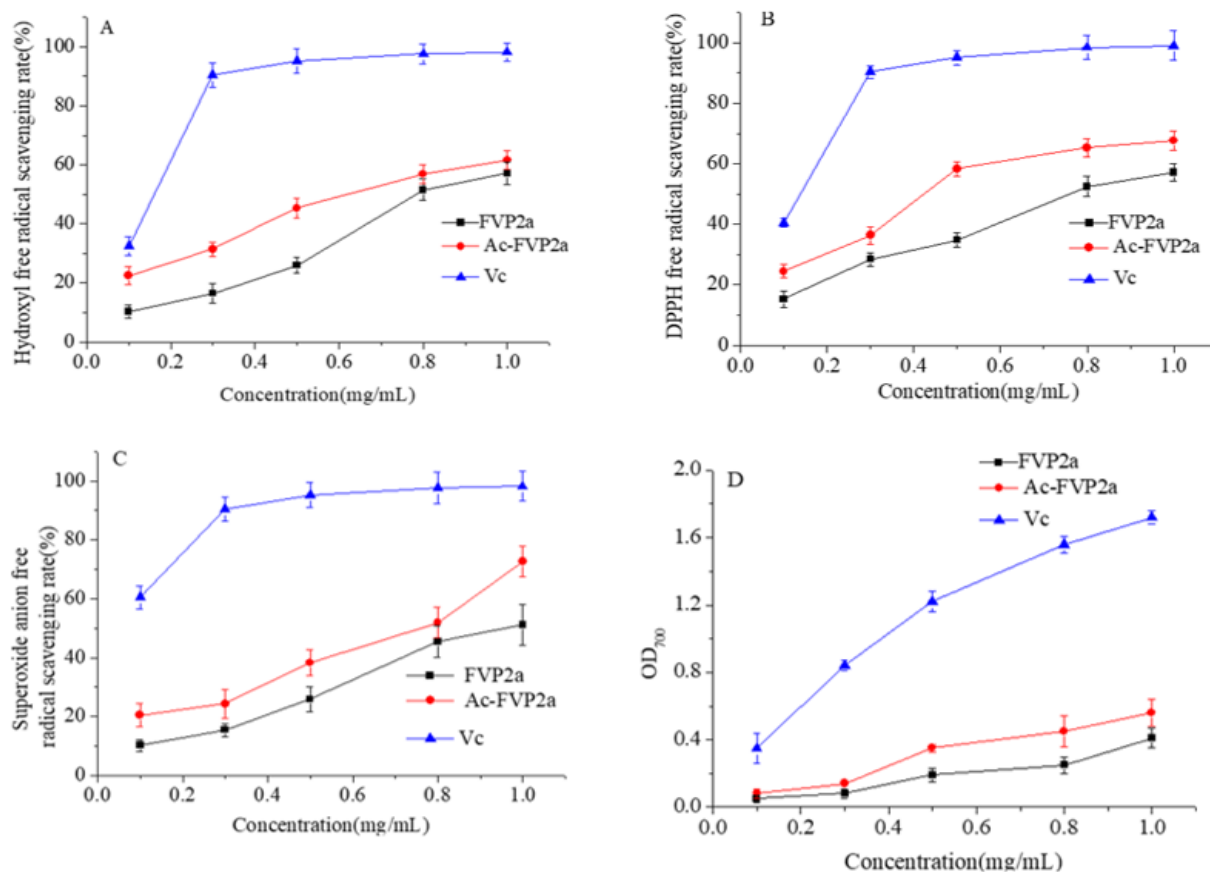
Fig. 3: Antioxidant activities in vitro of FVP2a and Ac-FVP2a. Hydroxyl radical (A), DPPH radical (B), Superoxide anion radical (C), and Reducing power (D)
